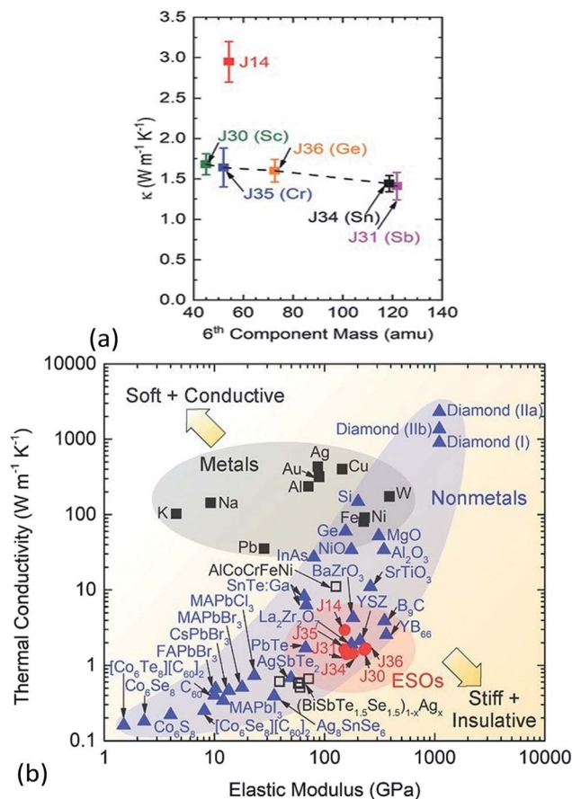
Fig. 7 (a) Thermal conductivity ( \kappa ) of six-cation MgCoNiCuZnXO 6 (X = Sc, Sb, Sn, Cr or Ge) high entropy oxides as a function of sixth atomic mass. The five-cation MgCoNiCuZnO 5 (J14 in red) is also shown at its average cation mass as a reference. (b) Thermal conductivity ( \kappa ) versus elastic modulus ( E ) for isotropic crystals at room temperature. The metals (squares) group has a subset of HEAs (open squares) and the non-metals (blue triangles) group has a subset of entropy stabilized oxides (ESOs, red circles). Reproduced with permission. Copyright 2018, John Wiley and Sons. 8
