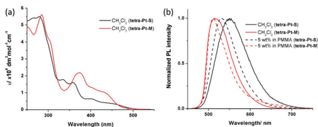
Fig. 1 (a) UV-vis absorption spectra and (b) PL spectra of tetra-Pt-S and tetra-Pt-M in \text{CH}_2\text{Cl}_2 and PMMA at room temperature.
