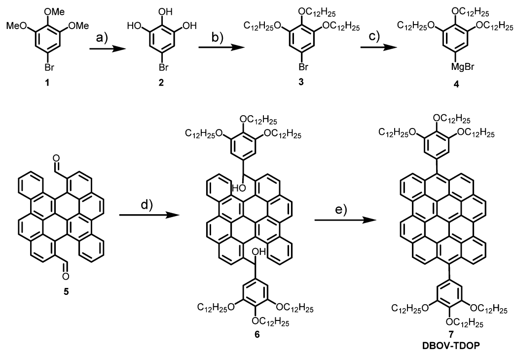
Scheme 1 Synthetic route towards 6,14-bis(3,4,5-tris(dodecyloxy)phenyl)dibenzo-[ hi, st ]ovalene ( DBOV-TDOP ). Reaction conditions: (a) BBr_3 , -78^\circ C to r.t., overnight, 98% yield; (b) C_{12}H_{25}Br , K_2CO_3 , N,N -dimethylformamide, 80^\circ C , 20 h, 63% yield; (c) Mg, I_2 , tetrahydrofuran, reflux, overnight; (d) 4 , tetrahydrofuran, 4 h, room temperature; (e) BF_3 \cdot OEt_2 , dichloromethane, room temperature, overnight, then p -chloranil, 2 h, 85% yield in three steps.
