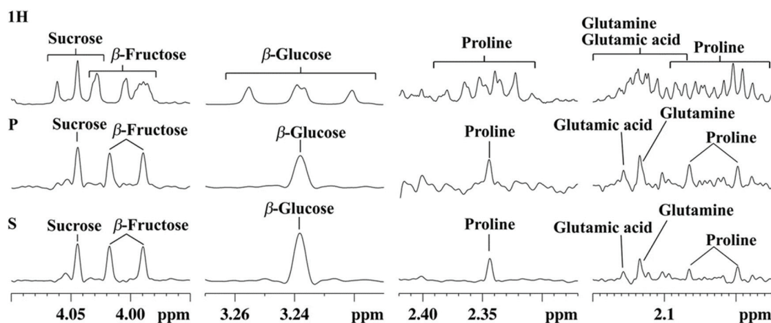
Fig. 3 Selected expansion regions of 1 H NMR (1H), PSYCHE (P), and SAPHIRE (S) spectra of an aqueous extract of Cape gooseberry ( Bambamarca l ) showing signal assignments. Figure reproduced from ref. 63 under Creative Commons Attribution 4.0 International License ( http://creativecommons.org/licenses/by/4.0/ ).
