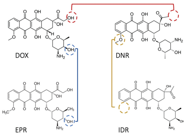
Fig. 1 Structures of the four most important and effective anthracyclines. Doxorubicin and daunorubicin contain a tetracyclic aglycone structure of four cyclohexane chains with a daunosamine sugar moiety. However, daunorubicin is seen with the absence of a hydroxyl group (red line). Compared with doxorubicin, epirubicin has an opposite chirality of the hydroxyl group in the daunosamine moiety (blue line). Idarubicin is identical to daunorubicin except the lack of 4-methoxy group on the ring (yellow line).
