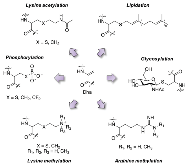
Fig. 4 Mimicry of post-translational modifications using dehydroalanine synthetic chemistry.
