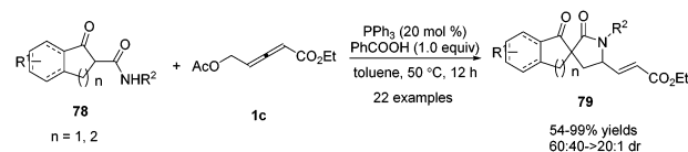
Scheme 25 \text{PPh}_3 -catalysed (3+2) spiroannulation of \alpha -substituted secondary \beta -ketoamides with \delta -acetoxy allenates.
