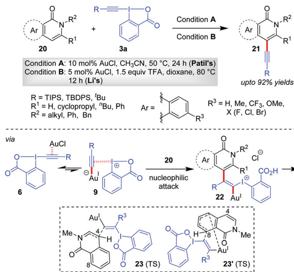
Scheme 5 Alkynylation of isoquinolones and 2-pyridones at the C4 site.
