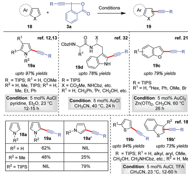
Scheme 4 Alkynylation of electron-rich heterocycles: pyrroles, thiophenes, benzofurans and tryptophan.
