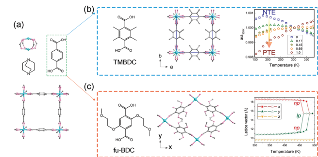
Fig. 8 (a) Crystal structure of the Zn 2 (BDC)(dabco) viewing along the c axis and its building units. (b) Illustration of the structure after TMDBDC decoration and the lattice parameter changes as a function of temperature and composition. (c) Illustration of the structure after fu-BDC decoration and the temperature-dependent lattice changes. Partly taken from ref. 70 and 71 with permission.
