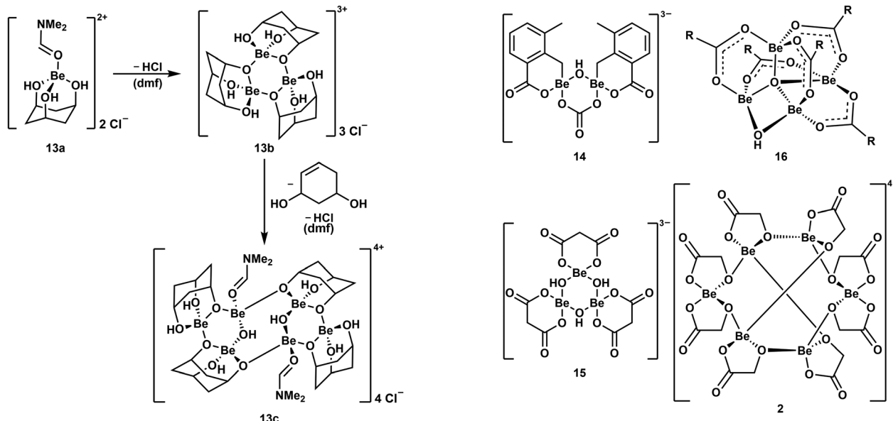
Fig. 8 Multinuclear beryllium compounds with bio-relevant ligands, which all contain six- or eight-membered beryllium heterocycles (R = 2-F-C 6 H 4 ). 39,41,57,58
