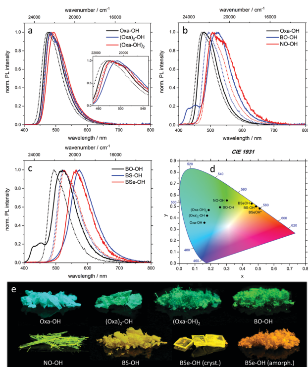
Fig. 2 (a–c) Normalized emission spectra of hydroxylated fluorenes measured for crystalline samples (solid lines) and as solution in chloroform (dotted lines). (d) CIE 1931 chromaticity plot with emission color coordinates of fluorenes in the solid-state. The amorphous sample is marked with an asterisk. (e) Representative images of hydroxylated fluorenes in the solid-state under 366 nm irradiation.
