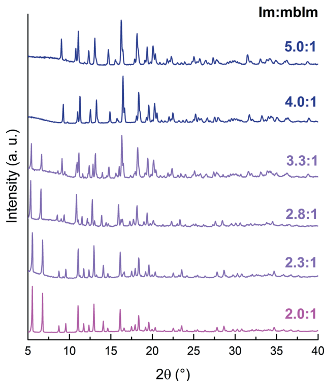
Fig. 5 Powder X-ray diffraction patterns of ZIF-76-mblm. Systematically increasing the Im:mbIm ratio in the ZIF-76-mblm synthesis from 2.0:1 to 5.0:1 gave sequentially pure ZIF-76-mblm (pink), mixed phase ZIF-76-mblm and TIF-4 (purple) then pure TIF-4 (dark blue).
