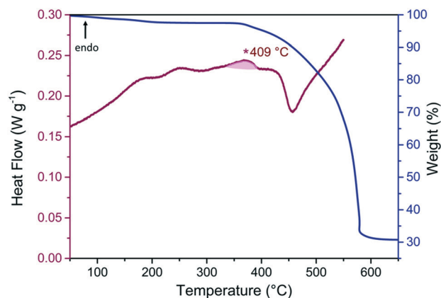
Fig. 6 TGA trace of ZIF-76-mblm (blue) with significant mass loss occurring above 400 °C. DSC trace of ZIF-76-mblm (pink) has an endothermic feature with an offset of 409 °C (marked by an asterisk and highlighted as a guide) followed by an exotherm associated with sample decomposition.
