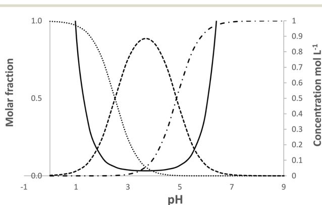
Fig. 5 Calculated speciation and solubility at 25 °C for p AHA in water in the pH range 0 to 9. Solid line solubility, ...protonated species, -.-.-, deprotonated species, ----neutral species.
