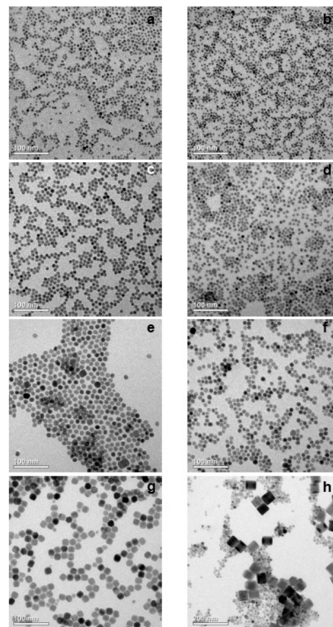
Fig. 3 TEM-images of \beta - \text{Na}_{1.5-2}\text{Sr}_x\text{Gd}_{1.5-2}\text{F}_6 nanoparticles with (a) x = 0.2 (b) x = 0.4 (c) x = 0.5 (d) x = 0.6 (e) x = 0.7 (f) x = 0.75 (g) x = 0.8 (h) x = 1 . For x = 1 , complete dissolution of the particles of the cubic phase was not achieved. A small amount of the cubic phase is also contained in the sample with x = 0.8 .
