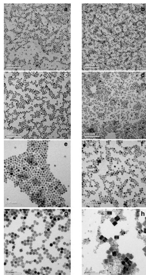
Fig. 3 TEM-images of \beta\text{-Na}_{1.5-3}\text{Sr}_x\text{Gd}_{1.5-3}\text{F}_6 nanoparticles with (a) x = 0.2 (b) x = 0.4 (c) x = 0.5 (d) x = 0.6 (e) x = 0.7 (f) x = 0.75 (g) x = 0.8 (h) x = 1 . For x = 1 , complete dissolution of the particles of the cubic phase was not achieved. A small amount of the cubic phase is also contained in the sample with x = 0.8 .
