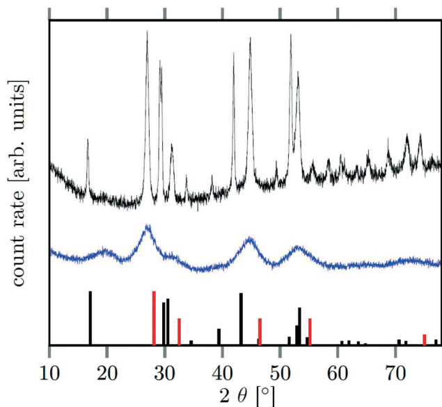
Fig. 2 XRD data of \text{Na}_{1.5-2}\text{Sr}_x\text{Gd}_{1.5-2}\text{F}_6 particles with x = 1 . Particles formed after heating for 45 min at 200 °C (blue), and after heating for 720 min at 320 °C (black). The vertical lines correspond to the reference patterns of \alpha - \text{NaGdF}_4 (red, ICSD-# 77099) and \beta - \text{NaGdF}_4 (black, ICSD-# 415868) respectively.
