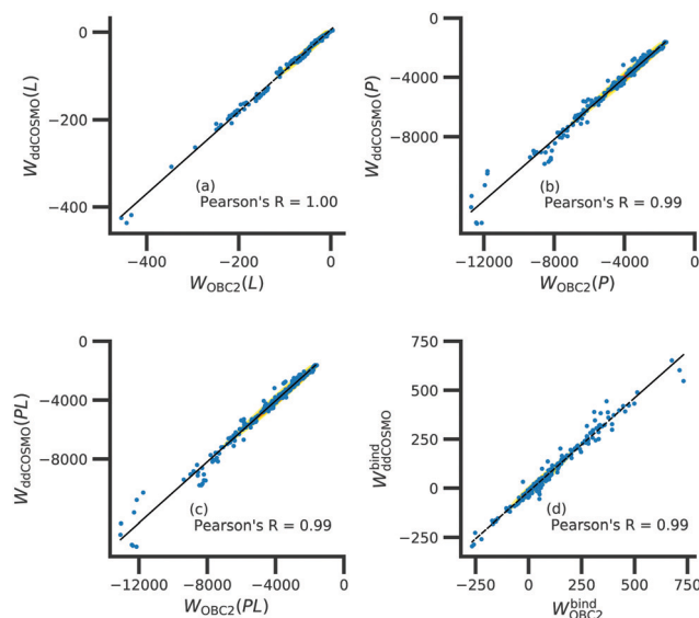
Fig. 10 Comparison of solvation free energy estimates (in kcal mol -1 ) based on OBC2 (x-axis) and ddCOSMO (y-axis). Solvation free energy estimates are of the (a) ligand, (b) protein, (c) complex, and (d) the binding energy.
