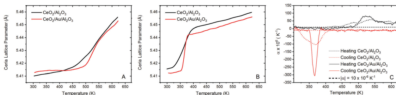
Fig. 3 Experimental DPDF results showing the extracted ceria lattice parameter. The ceria/alumina and ceria/Au/alumina ceria lattice parameter refinements are given in black and red respectively for experiments conducted during heating in a 5% \text{H}_2/\text{He} atmosphere for the heating (A) and cooling (B) in 5% \text{H}_2/\text{He} (C) instantaneous expansion coefficient during heating and cooling for the ceria/alumina (dotted lines) and ceria/Au/alumina (solid lines) samples. Dashed lines give the expected thermal expansion coefficient of ceria, \alpha = 10 \times 10^{-6} \text{ K}^{-1} , expansion in excess is associated to chemical change of the sample.
