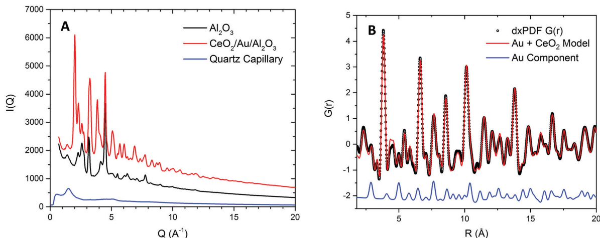
Fig. 2 Experimental DPDF patterns, alumina subtraction and Fourier Transformation recorded at room temperature. (A) Integrated total scattering pattern relating to: a ceria alumina support Au inverse catalyst sample, a gamma alumina support and fused quartz capillary sample environment; illustrating the process for correction to arrive at the differential xPDF containing the fluorite ceria and metallic Au components. (B) Example fit to the initial differential xPDF G(r) for a biphasic model containing fluorite ceria and metallic Au components over a fitting region of 1.8 to 20 Å. The metallic Au component contribution is highlighted below the data to illustrate the presence of the metallic Au phase within the extracted differential xPDF G(r) . Typical fit residual, r_w = 0.1 .
