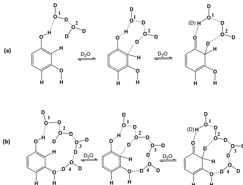
Fig. 8 Aromatic C–H activation of resorcinol in the presence of two (a) and four (b) bound molecules of \text{D}_2\text{O} .
