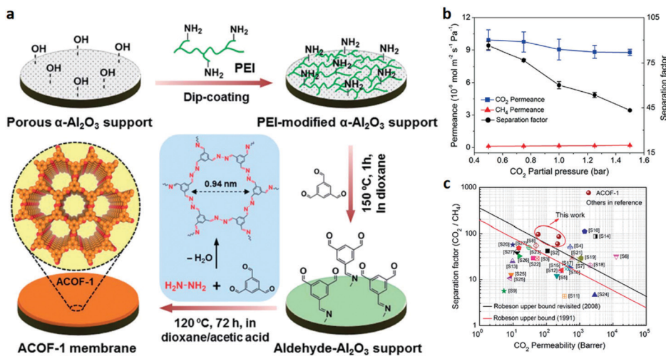
Fig. 15 (a) Schematic illustration of synthesizing the ACOF-1 membrane on the porous \alpha - \text{Al}_2\text{O}_3 support. (b) \text{CO}_2 permeance and \text{CO}_2/\text{CH}_4 separation factor of the ACOF-1 membrane as a function of the \text{CO}_2 partial pressure at 120 °C. (c) Permeability vs. separation factor of various membranes and the upper bound correlation for \text{CO}_2/\text{CH}_4 separation. Reproduced with permission from ref. 124. Copyright 2018, Royal Society of Chemistry.
