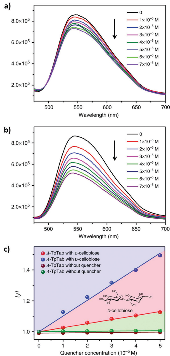
Fig. 26 (a and b) The fluorescence emission spectra of the (1)/(Δ)-TpTab COF with increasing concentration of the D-cellobiose quencher. (c) SV plots of the fluorescence emissions of the (1)/(Δ)-TpTab COF quenched by D-cellobiose. Adapted from ref. 88 with permission from Nature Research, copyright 2018.
