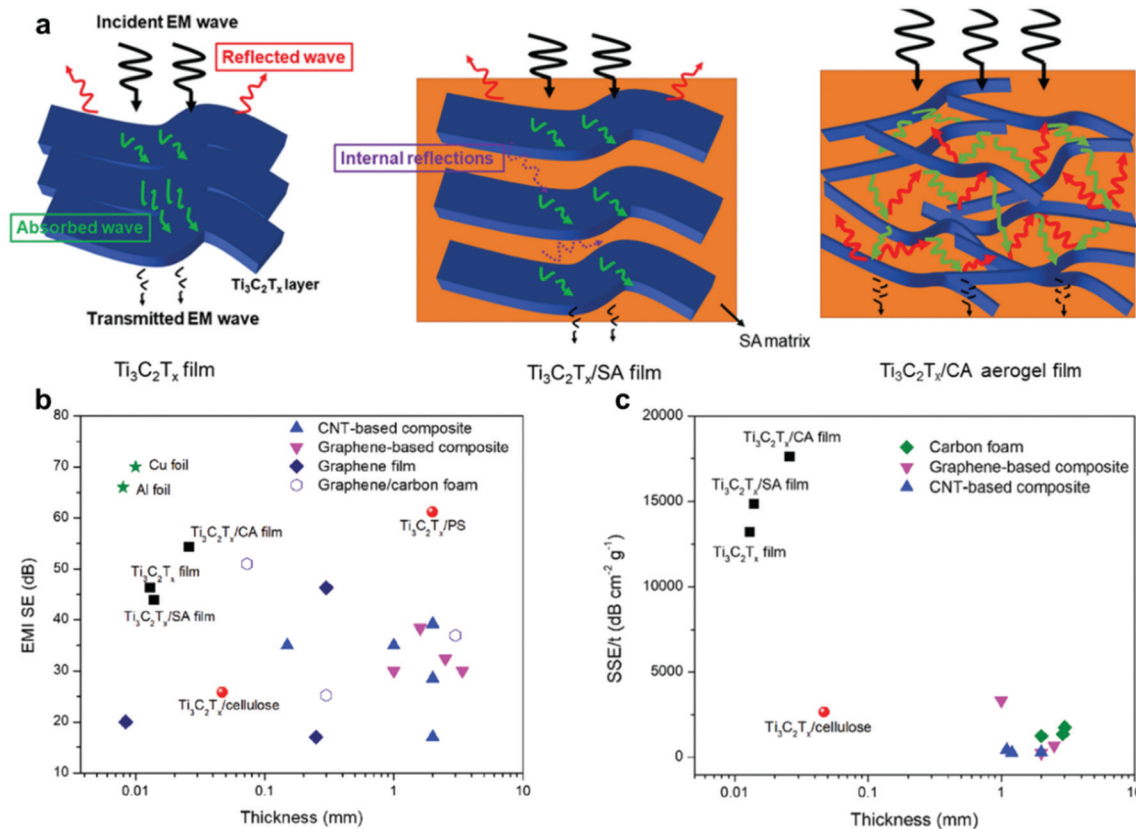
Fig. 15 (a) EMI shielding mechanism for freestanding Ti_3C_2T_x film, Ti_3C_2T_x/SA film, and Ti_3C_2T_x-CA aerogel. (b) Thickness-dependent EMI SE of various materials. (c) Different SSE/t at different sample thicknesses. Reproduced with permission from ref. 47 (copyright 2019, Wiley-VCH).
