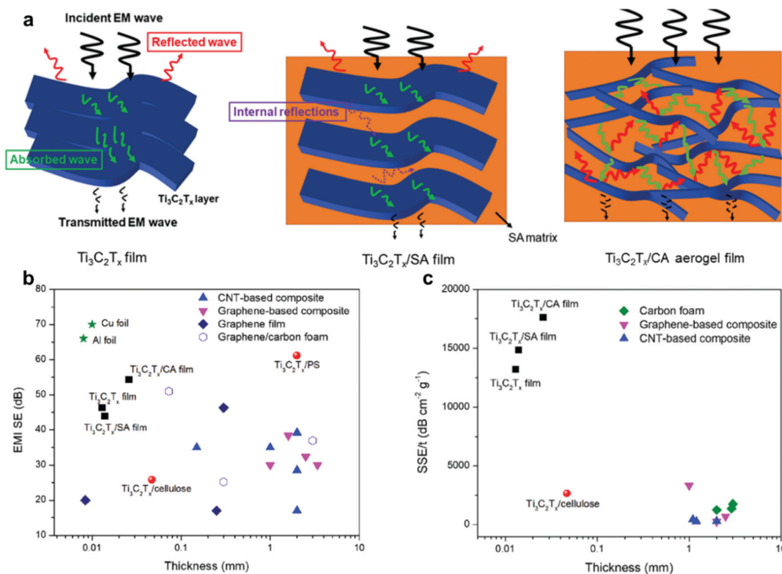
Fig. 15 (a) EMI shielding mechanism for freestanding Ti 3 C 2 T x film, Ti 3 C 2 T x /SA film, and Ti 3 C 2 T x -CA aerogel. (b) Thickness-dependent EMI SE of various materials. (c) Different SSE/t at different sample thicknesses. Reproduced with permission from ref. 47 (copyright 2019, Wiley-VCH).
