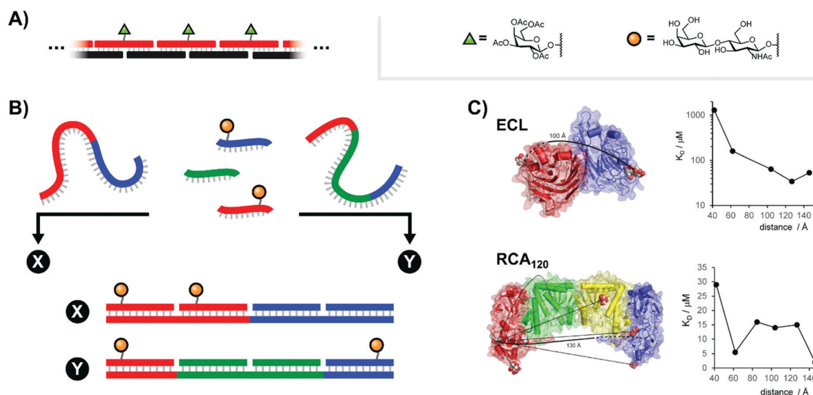
Fig. 3 Architectures of multivalent nucleic acid probes presenting carbohydrate ligands. (A) Repeating “half-sliding” formation for binding to Ricinus communis agglutinin (RCA 120 ) (ref. 8). (B) Tunable “molecular ruler” duplex design for targeting Erythrina cristagalli lectin (ECL) (ref. 10) or RCA 120 (ref. 12). By using different combinations of scaffold strands and ligand strands, constructs could be assembled with unique ligand arrangements (example: “X” vs. “Y”). (C) Crystal structures for ECL and RCA 120 depicting distances between binding sites as well as the distance-affinity curves obtained from the corresponding multivalent screening experiments (reproduced from ref. 13 with permission from John Wiley & Sons Inc., copyright 2019).
