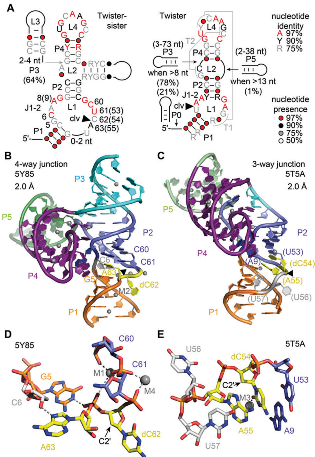
Fig. 10 Twister-sister ribozyme. (A) Secondary structure model of the consensus sequence of twister-sister (left) and comparison to twister (right). (B) Three-dimensional structure in cartoon presentation of the dC modified 4-way junctional (4WJ) ribozyme and (C) the dC modified 3-way junctional (3WJ) ribozyme. Note the differences at the cleavage site (yellow): splayed apart (dC62 and A63) for 4WJ, and stacked in double helix (dC54 and A55) for 3WJ. Black triangles indicate the cleavage positions. (D) Pocket for dC-A active site in the 2 structure of the 4WJ ribozyme with emphasis on the G5-scissile phosphate interaction. (E) Pocket for dC-A active site pocket in the structure of the 3WJ ribozyme.
