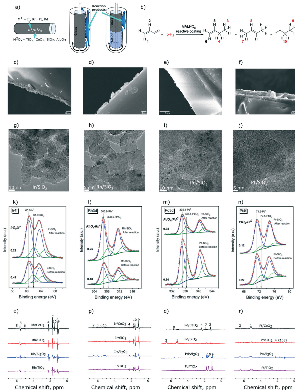
Fig. 1 a) Schematic representation of the reactors with catalytic coatings made of TiO 2 , CeO 2 , SiO 2 , and Al 2 O 3 containing Ir, Rh, Pt and Pd active phases (16 compositions in total) investigated in heterogeneous catalytic hydrogenation of b) 1,3-butadiene with p\text{-H}_2 (1:4 ratio). Photographs of reactive coatings with c) TiO 2 , d) CeO 2 , e) SiO 2 , and f) Al 2 O 3 with scale bars of 10, 1, 5 and 10 microns, respectively. Representative TEM images of the g) Ir/SiO 2 h) Rh/SiO 2 , i) Pd/SiO 2 , and j) Pt/SiO 2 reactive coatings. Deconvolution of k) Ir4f, l) Rh3d, m) Pd3d and n) Pt4f photoelectron spectra measured for silica-supported catalysts. 1 H NMR spectra obtained during hydrogenation of 1,3-butadiene at 130 °C using reactive coatings with o) Rh, p) Ir, q) Pd and r) Pt. The gas flow rate was 3.8 mL s -1 except for Rh/TiO 2 (5.1 mL s -1 ), Pd/SiO 2 (6.5 mL s -1 ) and Pd/TiO 2 (5.1 mL s -1 ).
