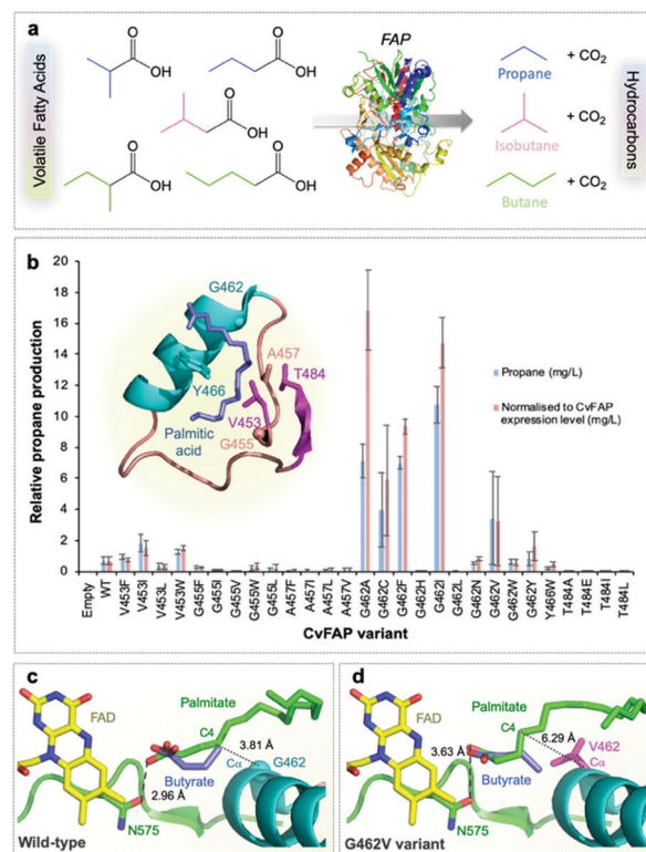
Fig. 1 Structure-guided molecular engineering of CvFAP. (a) Photo-catalytic gaseous hydrocarbon production from short chain volatile fatty acids. (b) Comparative propane production screen of variants of CvFAP in E. coli . Transformed E. coli cultures (three biological replicates) were grown at 37 °C in LB medium containing kanamycin (30 \mu\text{g mL}^{-1} ) to a density of OD 600 \sim 0.6–0.8. CvFAP expression was induced with IPTG (0.1 mM) and cultures were supplemented with 10 mM butyric acid. Triplicate aliquots (1 mL) of each culture were sealed into 5 mL glass vials and incubated at 30 °C for 16–18 h at 200 rpm, illuminated with a blue LED panel. Headspace gas was analysed for hydrocarbon content using a Micro GC. Data were normalized by dividing the propane titres ( \text{mg L}^{-1} culture) by the relative protein concentration compared to the wild type (WT) enzyme (Fig. S2; ESI†). Error bars represent one standard deviation for triplicate biological repeats ( n = 3 ). Inset: Structure of the palmitic acid binding region of CvFAP (PDB: 5NCC) shown as a cartoon with secondary structure colouring. Models of butyrate and palmitate in the active site of (c) wild-type and (d) G462V variant of CvFAP. The position of palmitate in the wild-type enzyme is crystallographically determined (PDB: 5NCC). The positions of the remaining ligands were determined by Autodock Vina, and mutagenesis to G462V was simulated using SwissPDBViewer 4.10. The protein is shown as a cartoon with secondary structure coloring, with selected residues shown as sticks. FAD, palmitate and butyrate are shown as atom-colored sticks with yellow, green and blue carbons, respectively. In panels c and d, the dashed line shows a hydrogen bond between palmitate and the wild-type enzyme, while the dotted lines indicate the distance between the C4 carbon of palmitate and the C \alpha atom of residue 462. All crystal structure images were generated in Pymol.
