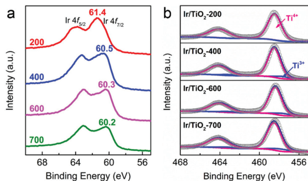
Fig. 5 (a) Ir 4f and (b) Ti 2p XP spectra of Ir/TiO 2-x catalysts.
