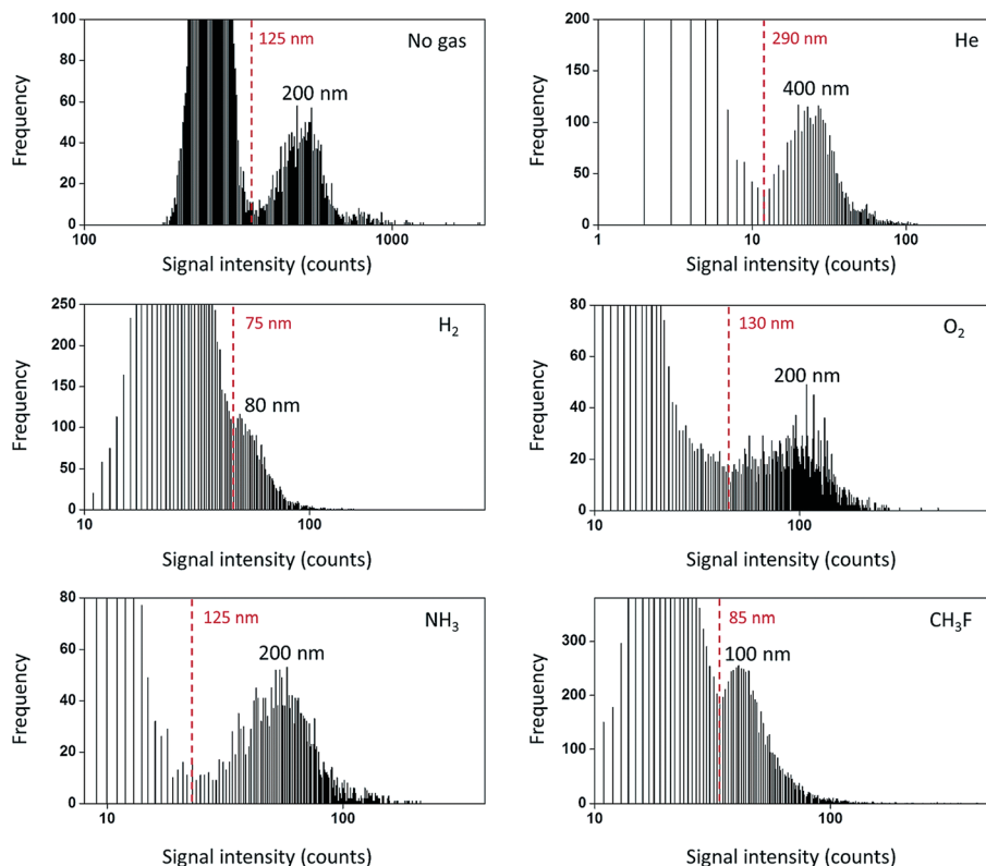
Fig. 4 Frequency distribution for the lowest NP sizes detectable using different reaction gases in ICP-TQ-MS for \text{SiO}_2 particle analysis. Practical \text{LODs}_{\text{size}} are indicated in red in each figure. Frequency refers to the number of events of each type (background or NPs) detected. Reproduced from Bolea-Fernandez et al. 56 with permission from the Royal Society of Chemistry.
