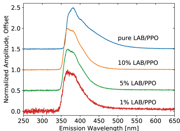
Fig. 2 Emission spectra resulting from X-ray excitation of pure LS (LAB with 90 \text{ g L}^{-1} PPO) and the three WbLS concentrations made from this LS. Each curve is displayed normalized at its maximum and offset along the vertical axis.
