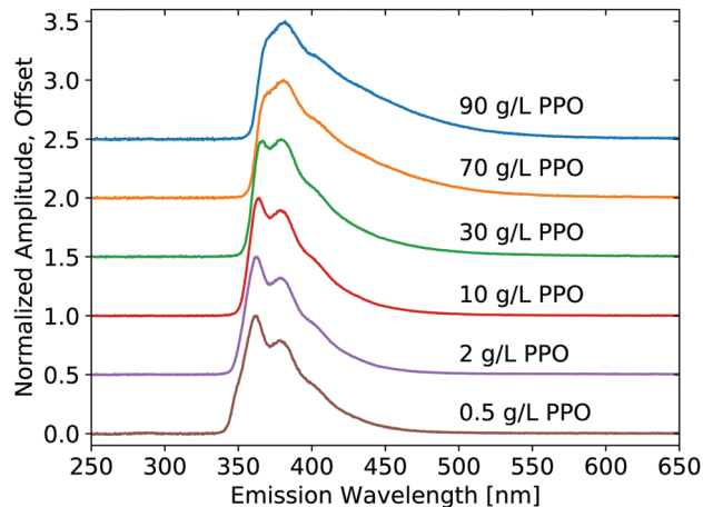
Fig. 1 Emission spectra resulting from X-ray excitation of pure LS with varying concentrations of PPO in LAB. Each curve is displayed normalized at its maximum and offset along the vertical axis.
