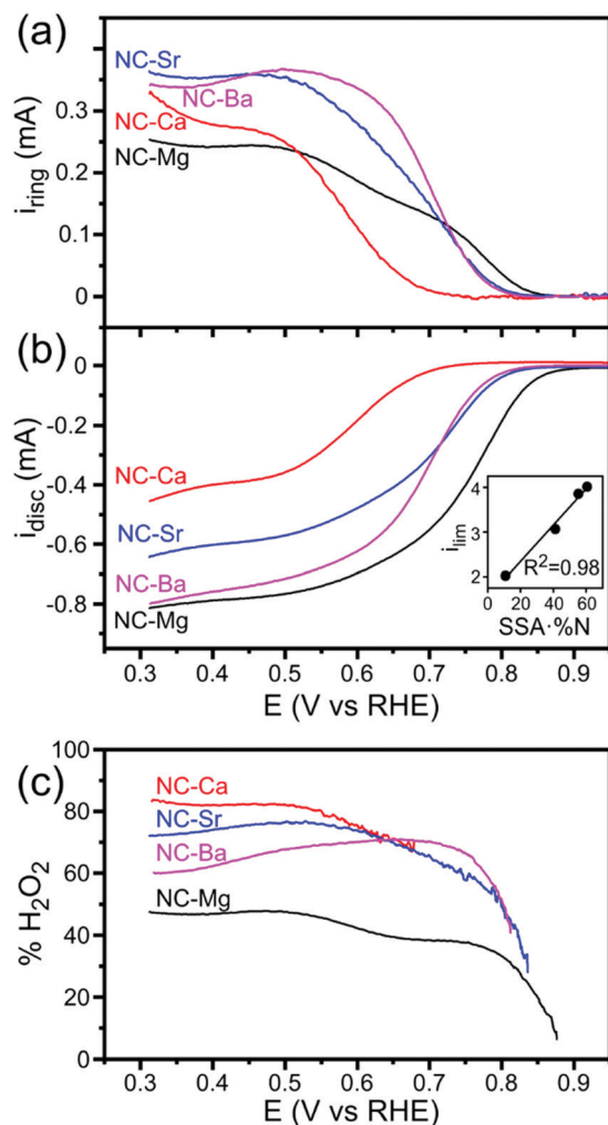
Fig. 11 Linear scan RRDE voltammograms of O_2 -saturated 0.1 M KOH at 25 °C, scan rate at 10 mV s^{-2} , rotated at 1600 rpm, corrected for capacitive current as measured in a N_2 -purged solution. (a) Ring current, corrected by the collection factor. (b) Disc current. Inset: Limiting disc current ( -0.6 V vs. RHE) vs. number of N atoms per specific surface area of the carbon (see text). (c) Calculated percent of produced H_2O_2 .
