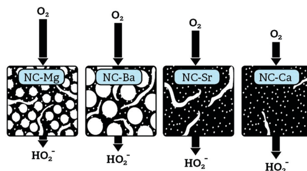
Fig. 13 Proposed mechanism for the observed structure–activity correlations in the NC-M carbons: hierarchical porosity enables better O_2 delivery into the particles, while confinement of peroxide in mesopores allows it to react more completely.
