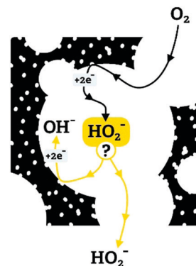
Fig. 12 Proposed mechanism for the observed ORR selectivity differences, based on competition between kinetics and mass transfer. The peroxide ( HO_2^- ) intermediate can either escape (from large pores) or be reduced/disproportionated (if confined in small pores).
