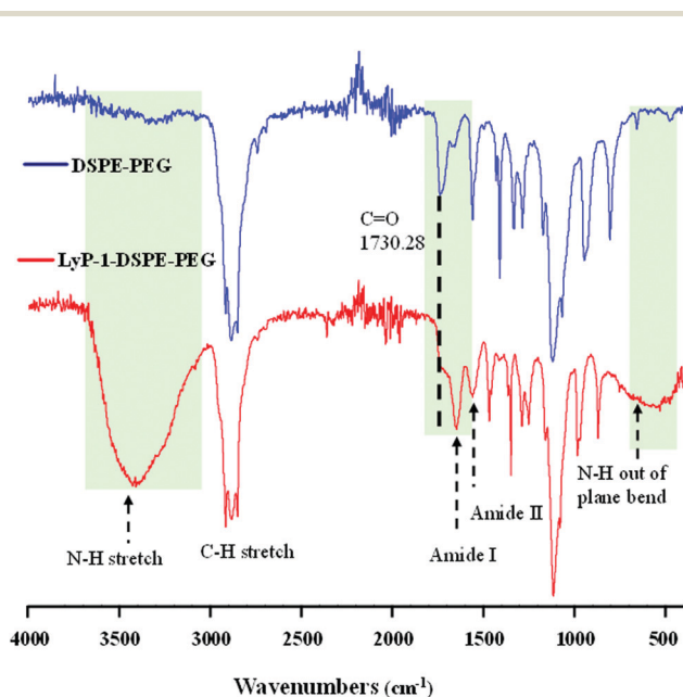
Fig. 1 Chemical characterization of synthesized LyP-1–DSPE–PEG using an FT-IR spectrum showing the functional peaks of the starting materials (DSPE–PEG) and product (LyP-1–DSPE–PEG). The LyP-1–DSPE–PEG spectrum was obtained with the lyophilized product.
