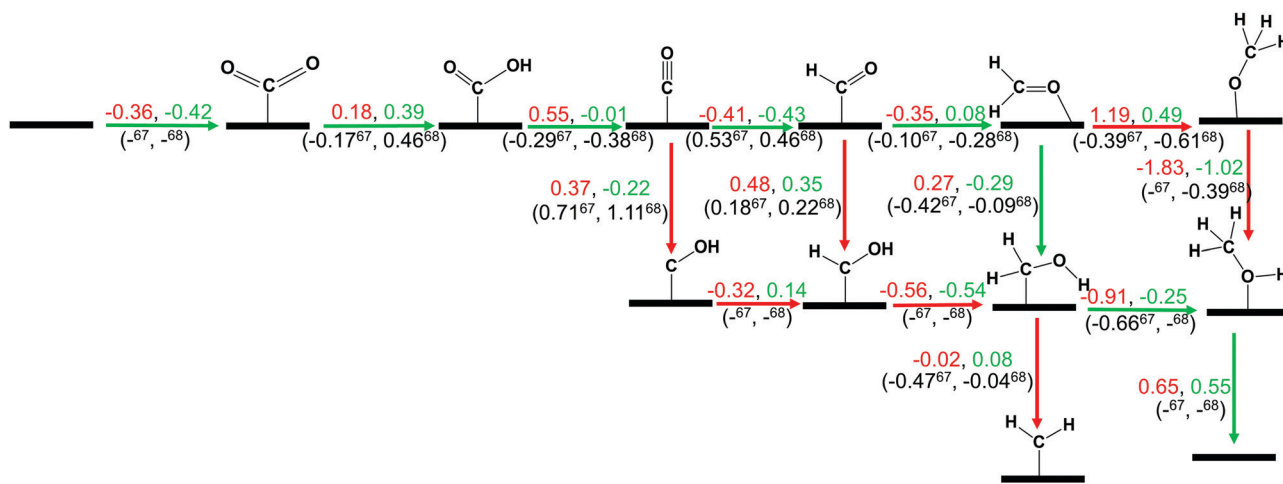
Scheme 1 The calculated ZPE corrected reaction energies (eV) for electrochemical CO 2 hydrogenation reaction on ZnO (red) and Cu@ZnO (green) NCs. Our calculated ZPE corrected reaction energies are compared with those of the previous reports on the Cu nanocluster and Cu(111) ML. 67,68 Here, (-) means that the energy is not available for this step. The green arrow shows the most favourable pathway for the CO 2 hydrogenation reaction to CH 3 OH.
