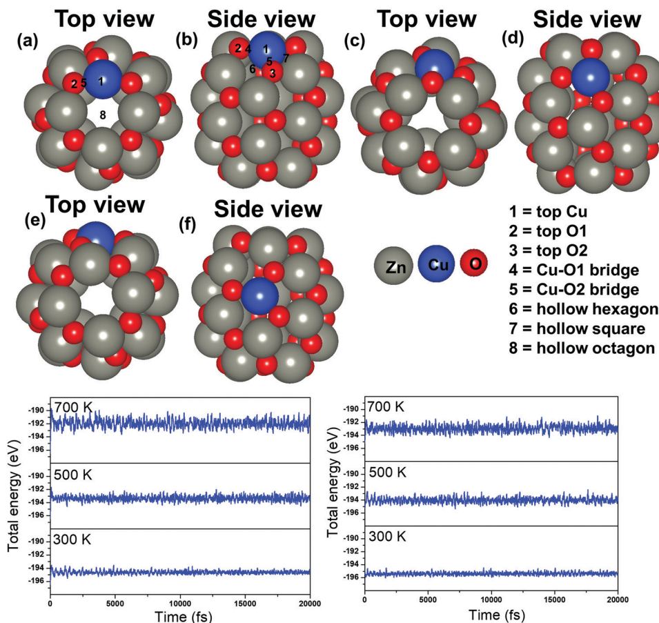
Fig. 2 Top and side views of considered Cu doped ZnO NCs: (a and b) first layer Cu doped Zn 24 O 24 , (c and d) second layer Cu doped Zn 24 O 24 , and (e and f) third layer Cu doped Zn 24 O 24 . (g and h) Ab initio molecular dynamics simulations of (g) ZnO and (h) Cu@ZnO NCs at 300, 500 and 700 K.
