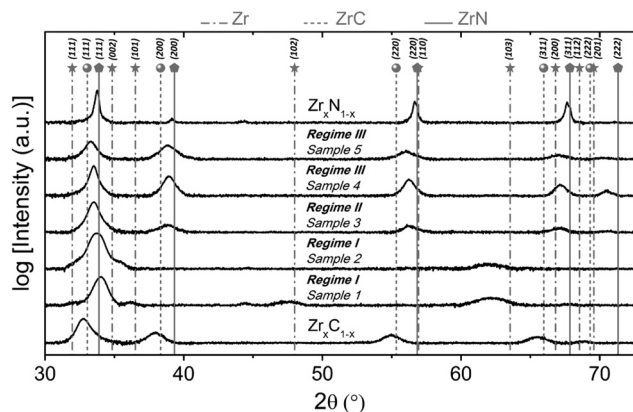
Fig. 6 XRD spectra of ZrCN coatings developed from various regimes. (Reprinted from ref. 137 with permission from Elsevier.)
