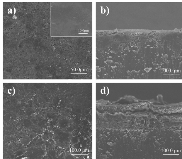
Fig. 7 SEM images of the LFPP-Li anode (a, top view; b, side view) and the polished Li anode (c, top view; d, side view) after cycling in Li/LiFePO 4 cells for 500 cycles at 0.5C.
