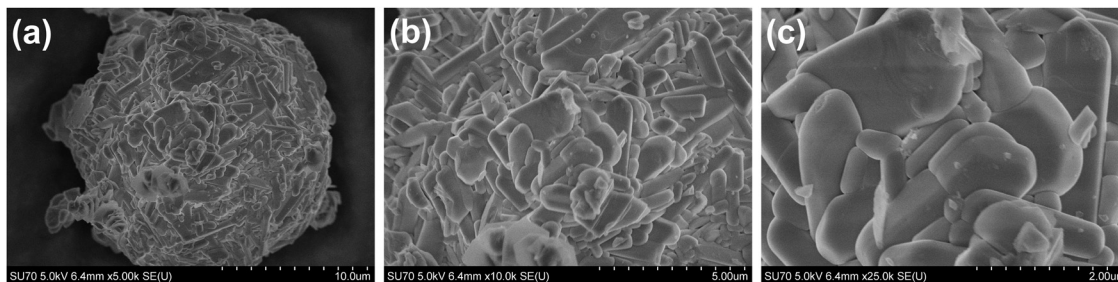
Fig. 2 SEM images of \text{K}_2\text{Bi}(\text{PO}_4)(\text{MoO}_4):50\%\text{Sm}^{3+} powder at different magnifications.
