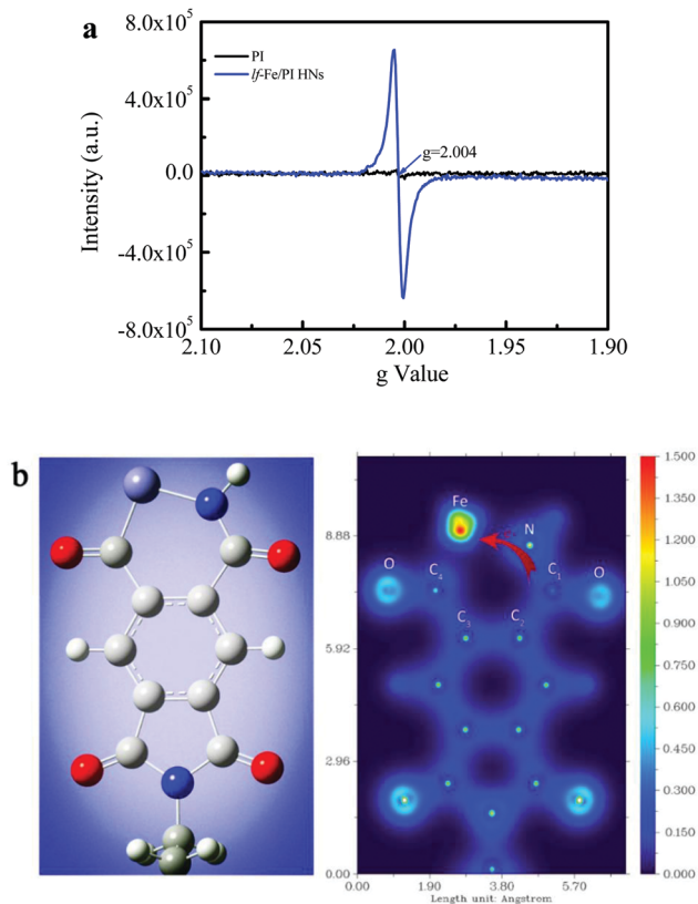
Fig. 4 Non-uniform distribution of surface electrons on If-Fe/PI HN. (a) EPR spectra of PI and If-Fe/PI HN. (b) DFT calculations for the optimized structure of If-Fe/PI HN in one unit (left) and the corresponding two-dimensional valence-electron density color-filled maps of the If-Fe/PI HN model (right). Purple, red, grey and blue circles denote Fe, O, C and N atoms, respectively. The valence-electron density is given in e \text{ \AA}^{-3} .
