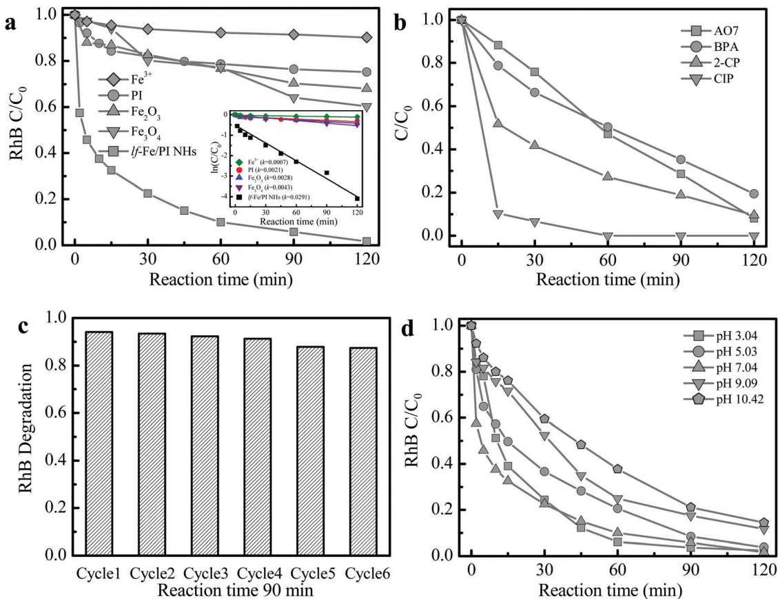
Fig. 5 Performance of lf-Fe/PI HN for pollutant removal. (a) RhB degradation curves in various suspensions with H 2 O 2 (inset shows the corresponding kinetic curves). (b) Decomposition curves of other different pollutants in the lf-Fe/PI HN suspensions with H 2 O 2 . (c) Reusability of lf-Fe/PI HN for RhB degradation. (d) Effect of initial pH values for RhB degradation. Reaction conditions: natural initial pH (pH 6–7, except (d)), initial pollutants 10 mg L -1 , initial H 2 O 2 10 mM, catalyst 1.0 g L -1 (Fe ions 0.15 mg L -1 in (a)).
