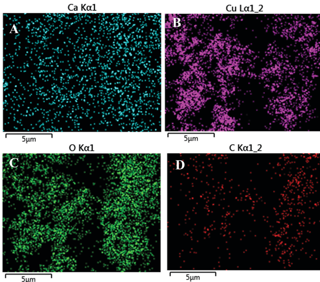
Fig. 4 Energy dispersive X-ray mapping of the \text{CaCu}_2\text{O}_3\text{-200} sample annealed at 200 °C in air.
