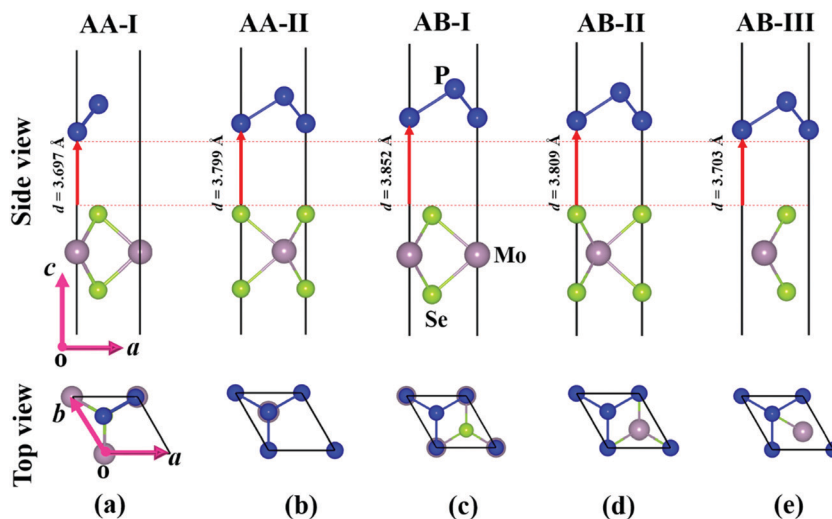
Fig. 1 Optimized structures of P_2/MoSe_2 vdW heterostructures with different stacking configurations: (a) AA-I, (b) AA-II, (c) AB-I, (d) AB-II, and (e) AB-III.
