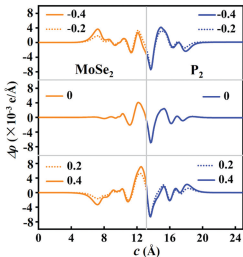
Fig. 6 Planar-averaged electron density difference across the P_2/\text{MoSe}_2 vdW heterostructure under various electric fields of -0.4 \text{ V \AA}^{-1} , -0.2 \text{ V \AA}^{-1} , 0 \text{ V \AA}^{-1} , 0.2 \text{ V \AA}^{-1} , and 0.4 \text{ V \AA}^{-1} . The orange (blue) region corresponds to the MoSe 2 ( P_2 ) layer.
