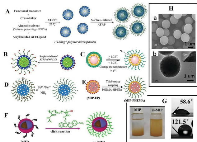
Fig. 3 Representation of MIPs with polymer brush. (A) A scheme for preparation of spherical MIPs with polymer brushes by living polymerization, adapted from ref. 72, Copyright 2012. (B) Fluorescent MIPs with brush, adapted from ref. 77, Copyright 2016 American Chemical Society. (C) Multi-responsive MIPs, adapted from ref. 71, Copyright 2012. (D) Magnetic MIPs with brush, adapted from ref. 74, Copyright 2014. (E) Preparation of MIPs with brush by thiol epoxy coupling, adapted from ref. 79, Copyright 2019. (F) Polymer brush by click reaction, adapted from ref. 81, Copyright 2020 American Chemical Society. (H) Images of MIPs with polymer brush (a) adapted from ref. 78, Copyright 2012; and (b) adapted from ref. 74, Copyright 2014. (G) The water contact angle and the dispersity of MIPs in water, adapted from ref. 81, Copyright 2020 American Chemical Society.
