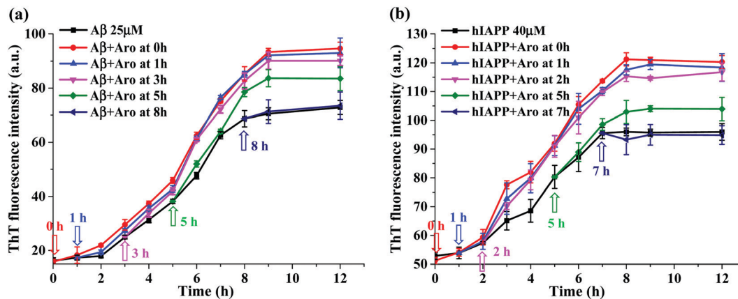
Fig. 6 Time-dependent ThT fluorescence profiles by addition of equimolar aromadendrin to (a) A \beta_{42} (25 \mu M)- and (b) hIAPP 37 (40 \mu M)-seeded solutions at different time points. Arrows indicate the time points of addition of aromadendrin to the amyloid-seeded solutions. Error bars represent the average of three replicate experiments.
