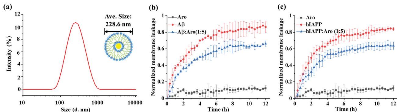
Fig. 8 Effect of aromadendrin on membrane leakage. (a) Size distribution of as-prepared large unilamellar vesicles (LUVs). Comparison of (b) A \beta - and (c) hIAPP 37 -induced membrane leakage in the absence and presence of aromadendrin at an amyloid : aromadendrin molar ratio of 1 : 5 (25 \mu M : 125 \mu M). Data represent mean \pm s.d. of three independent experiments ( n = 3 ). The time-dependent membrane leakage in the presence of amyloid or amyloid : aromadendrin (1 : 5) was analyzed by two-way ANOVA. Comparison of membrane leakage between amyloid : aromadendrin (1 : 5) and pure amyloid samples revealed a P value < 0.01 .
