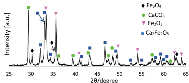
Fig. 1 XRD pattern for FS-processed \text{Fe}_3\text{O}_4\text{:CaCO}_3 .
