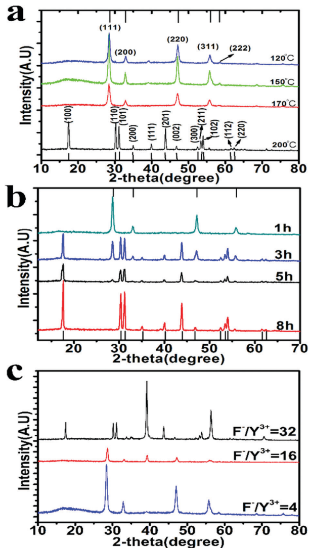
Fig. 3 (a) XRD spectra of the UCNs obtained at different reaction temperatures for 8 h. PDF (no. 01-077-2042) of cubic \alpha -phase and PDF (no. 00-016-0334) of hexagonal \beta -phase \text{NaYF}_4 are indicated at the top and bottom axis, respectively. (b) XRD spectra of the UCNs prepared using different reaction durations at 200 °C. (c) XRD spectra of the UCNs prepared at 150 °C for 7 h with different \text{F}^- to \text{Y}^{3+} molar ratios.
