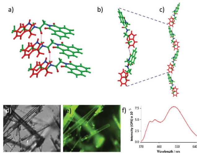
Fig. 1 (a) Amide hydrogen bonding mediated J-type aggregation of NMI-GW-OMe in the solid-state. (b) Head to tail interactions of two NMI derivatives through \text{C-H}\cdots\text{O} hydrogen bonding interactions (oxygen of the naphthalimide unit and tryptophan ring hydrogen). (c) Formation of a helical structure in the solid-state. (d) Optical and (e) fluorescence microscopic images of NMI-OMe crystals and (f) solid-state fluorescence spectra of NMI-GW-OMe at 30^\circ\text{C} .
