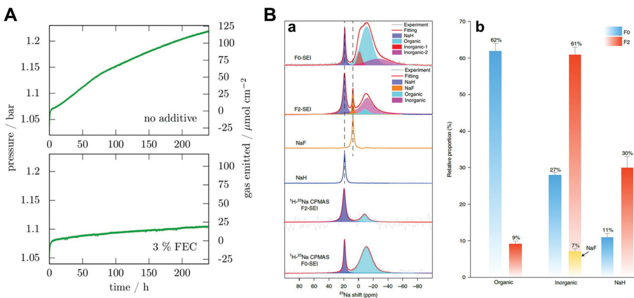
Fig. 6 (A) Pressure variation in a 9.2 cm 3 cell containing a 0.5 cm 2 sodium electrode and 250 \mu\text{L} electrolyte without the additive and with 3% FEC in mass. Reproduced with permission from ref. 70. Copyright 2016, Electrochemical Society. (B) Ex situ NMR characterization of the SEI species. (a) Single-pulse 23 Na NMR and 1 H \rightarrow 23 Na CPMAS NMR spectra of SEI species harvested from Cu foil after 50 cycles and the reference spectra of NaF and NaH. (b) The relative proportion of organic and inorganic components in the SEI species. Error bars indicate errors when fitting the NMR signals of different SEI components. Reproduced with permission from ref. 51. Copyright 2020, Springer Nature.
