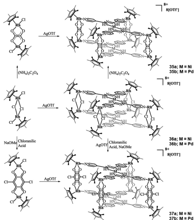
Scheme 14 The synthetic routes that led to the isolation of the organometallic heterometallic complexes, where M = \text{Ni}^{\text{II}} or \text{Pd}^{\text{II}} . Adapted with permission from ref. 54. Copyright 2017 Royal Society of Chemistry.
