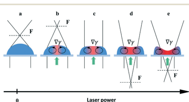
Fig. 2 Schematic illustration of the droplet reshaping by the thermocapillary forces induced with the laser beam. The axis shows the laser power increase. \nabla\gamma is the thermal surface tension gradient along the liquid interface. (a) The initial shape of the droplet (the laser is off); (b) the flattening of the droplet surface – the focal length increases (the laser is on); (c) the droplet with the flat surface – the focal length tends to infinity; (d) and (e) the formation of thermocapillary dimple in the droplet, negative focal length.
