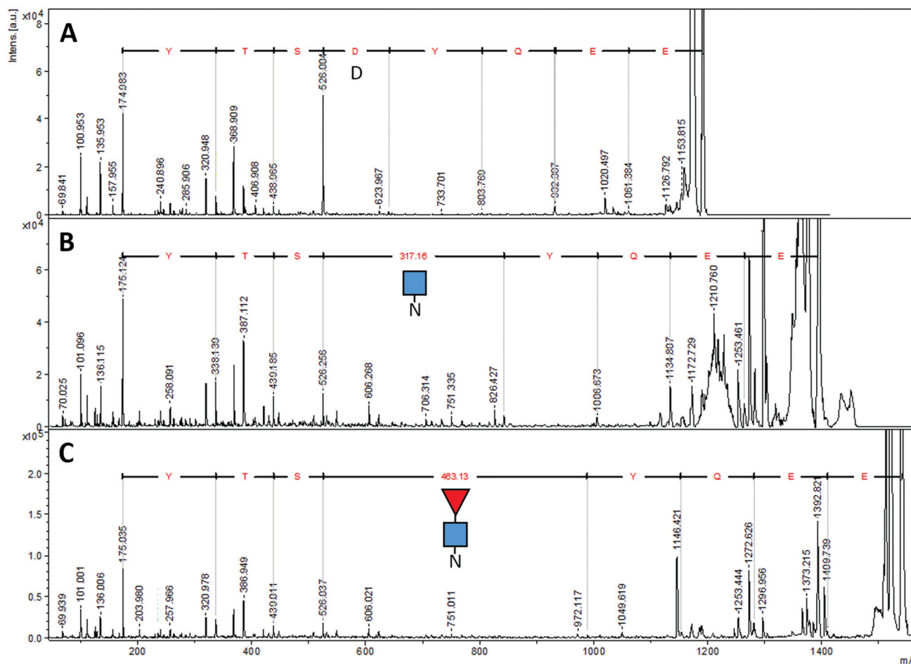
Fig. 6 MALDI-MS/MS spectra of different forms of EG2-hFc's tryptic peptide EEQYNSTYR. (A) After PNGase F deglycosylation, (B) with only GlcNAc attached, (C) with GlcNAc–Fuc attached. The \Delta m/z values of 317.16 and 463.13 correspond to Asn + GlcNAc and Asn + GlcNAc–Fuc, respectively. Ions at m/z 175 are y_1 ions of arginine (R). Sequencing was performed using the series of y fragments in each case. ■ GlcNAc, ▲ fucose, N asparagine, D aspartic acid.
