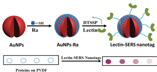
Fig. 1 Schematic illustration of the fabrication of lectin-SERS nanotags and the assay for rapid glycoprotein identification and quantification. The Raman reporter MBA binds to the AuNPs surface via a thiol group. Lectin is attached to the AuNPs surface using the DTSSP crosslinker, yielding the lectin-SERS nanotag. An assay is performed by immobilising glycoproteins on a PVDF membrane, which is then incubated with the lectin-SERS nanotags. Binding of the nanotags indicates the presence of the lectin's target glycans on the immobilised protein. This is detected with a Raman microscope, where signal intensity correlates with abundance of the target glycans.
