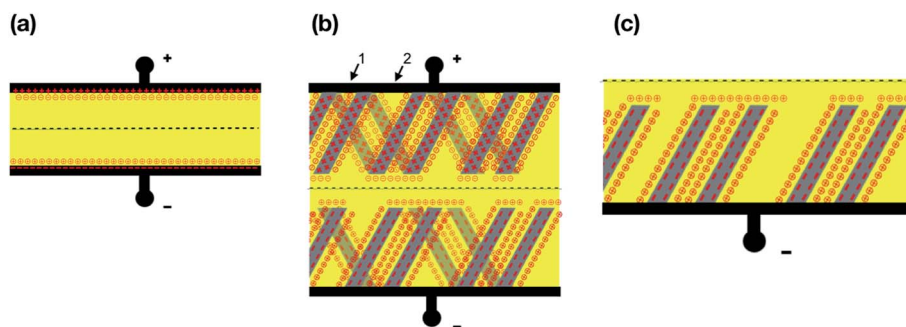
Fig. 10 (a) Schematic view of a charged capacitor (left) and (b) supercapacitor (right): solid black—electrodes; dashed—separator; yellow—electrolyte; nanotubes schematically shown in shades of gray; numbers indicate the hierarchical system of pores 1—small pores and 2 big ones; “+”—positive charge; “ \ominus ”—negative ion; “-”—negative charge (electrons); “ \oplus ”—positive ion. (c) Illustration of a part of a supercapacitor consisting of monolayers of nanotubes. 167
