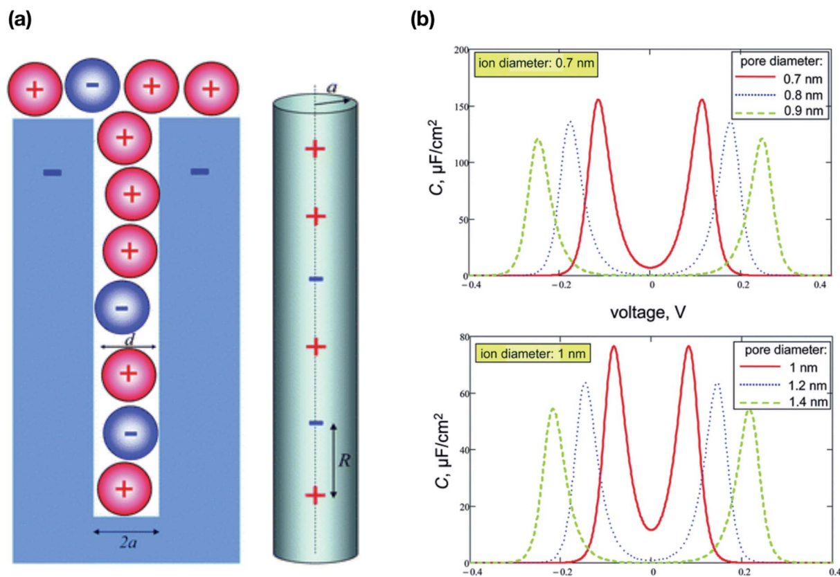
Fig. 8 (a) Schematic cross section of a negatively polarized electrode pore showing accommodation of one line of ions in the order of d < 2a < 2d . One dimensional lattice representation of distribution of ions. Reprinted with permission from Royal Society Publishing. 73 (b) The specific voltage-dependent differential capacitance of a single pore per unit surface area. The effect of the diameter of the pore, shown for an ion diameter of 0.7 nm (upper panel) and 1 nm (lower panel); the effective dielectric constant of the pore interior, \epsilon = 2 . Due to saturation of charge density, the capacitance vanishes very quickly with voltage. (a and b) have been adapted/reproduced from ref. 73 with permission from the Royal Society of Chemistry. 73
