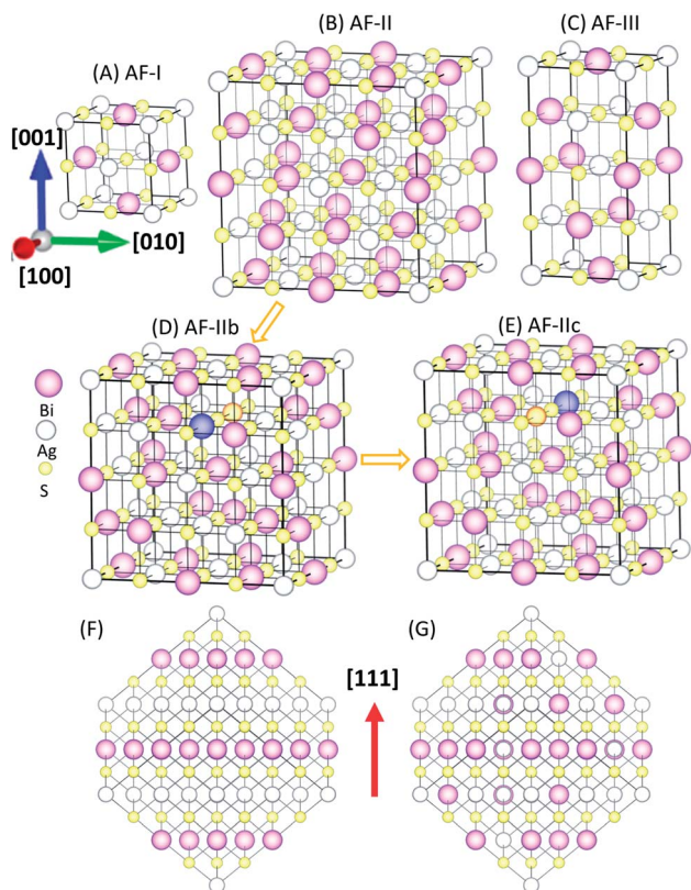
Fig. 1 Possible ordered structures of AgBiS 2 : (A) AF-I (space groups: P4/mmm ), (B) AF-II ( R3m ), (C) AF-III ( I4_1/amd ), (D) AF-IIb ( F3dm ), and (E) AF-IIc ( C2/m ). (F) AF-II viewed in the direction normal to [111]. (G) AF-IIb viewed in the direction normal to [111]. Indigo and orange balls denote the swapped Bi and Ag sites from AF-IIb to AF-IIc.
