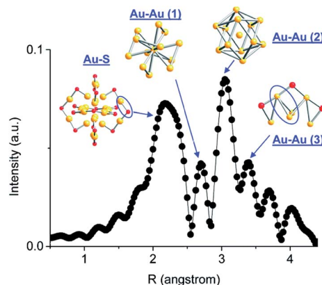
Fig. 2 Simulated FT-EXAFS of \text{Au}_{25}(\text{SR})_{18} clusters. The simulation was done by averaging the EXAFS from all representative Au sites of \text{Au}_{25} ( k : 3\text{--}14.5 Å -1 , k^1 weighted). The spectrum was phase-corrected using the Au–S peak. Reprinted with permission from ref. 43. Copyright 2011, American Chemical Society.
