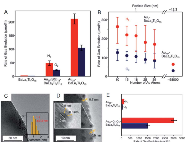
Fig. 10 Effect of (A) ligands protection and (B) cluster size on the rates of photocatalytic activity for water splitting studied using Au n /BaLa 4 Ti 4 O 15 ( n = 10\text{--}39 ) and Au NPs/BaLa 4 Ti 4 O 15 . (C) TEM image. (D) High resolution-TEM image. (E) Rates of photocatalytic activity for water splitting of Au 25 -Cr 2 O 3 /BaLa 4 Ti 4 O 15 . Panels (a) and (b) are reproduced with permission from ref. 60. Copyright 2015 American Chemical Society. Panels (c)–(e) are reproduced with permission from ref. 61. Copyright 2018 American Chemical Society.
